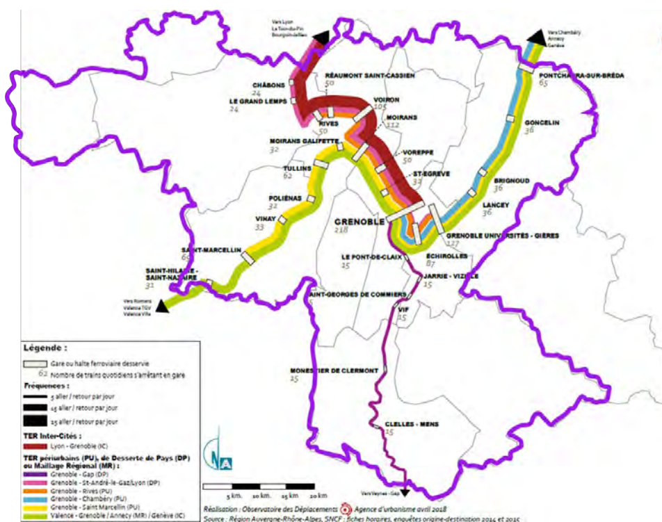
Figure 31 : TER (Source : ASTER GDEM product of METI and NASA, traitement AURG)
